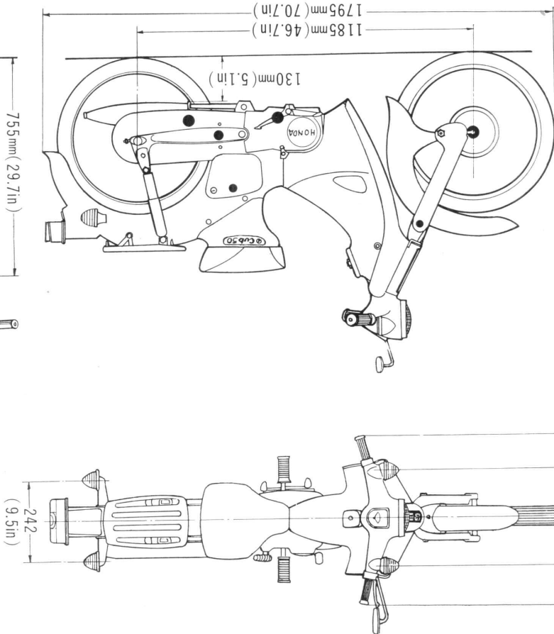
DIMENSIONAL DRAWING
