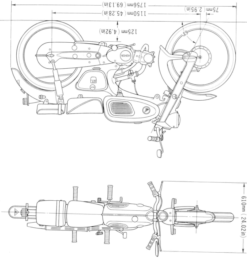
DIMENSIONAL DRAWING
