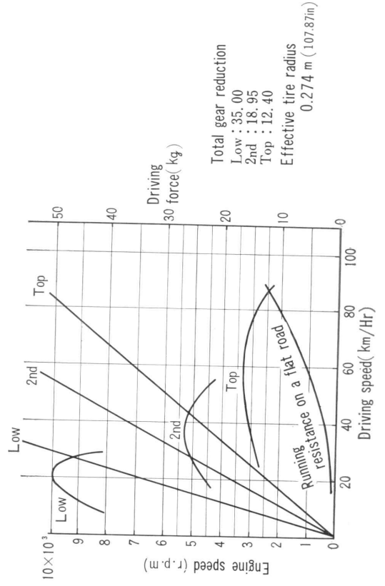
Running Performance (C 65 M)
