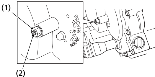
(1) lock nut
