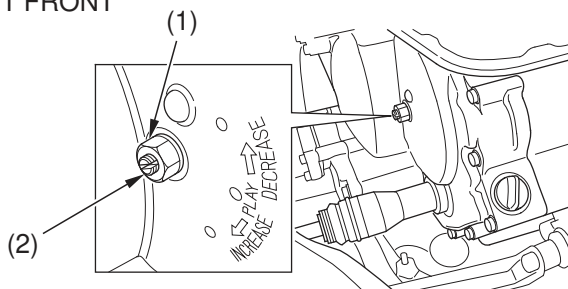
(1) lock nut
