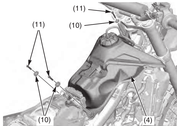
(4) fuel tank (10) washers (11) fuel tank bolts
