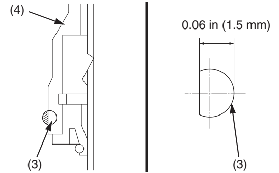
(3) wear rings
