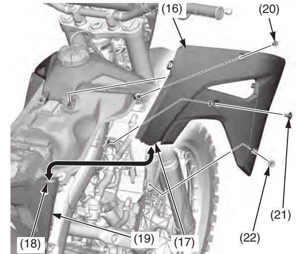
(16) shroud (20) shroud C bolt (17) tab (21) shroud B bolt (18) slot (22) shroud A bolt (19) side cover
