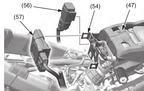
(47) seat support base (56) starter relay (54) ECM stay (57) ECM
