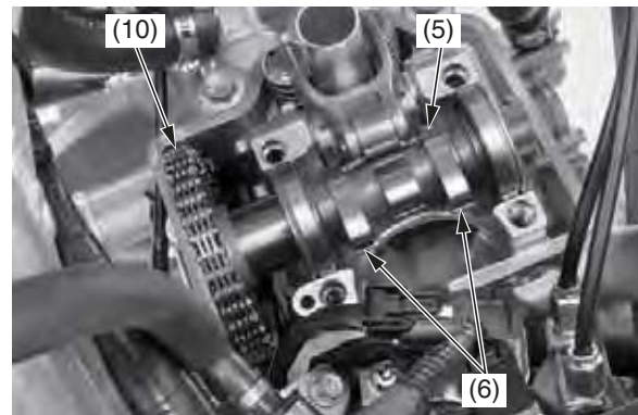
(5) camshaft (6) intake cam lobes (10) cam chain
