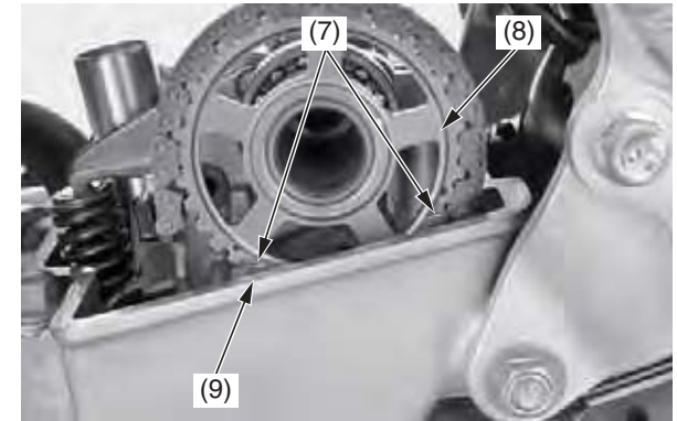
(7) timing marks (8) cam sprocket (9) surface of the cylinder head
