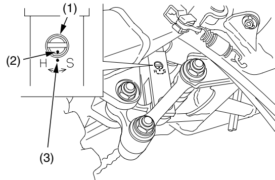
(1) rebound damping adjuster (3) reference mark (2) punch mark
