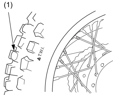
(1) tread depth
