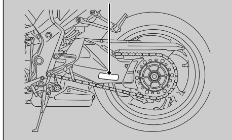
Vehicle emission control information label
