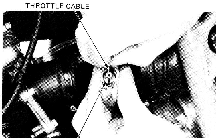
CABLE HOLDER
