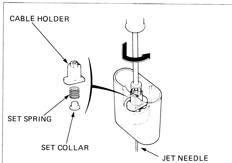
CARBURETOR TOP
