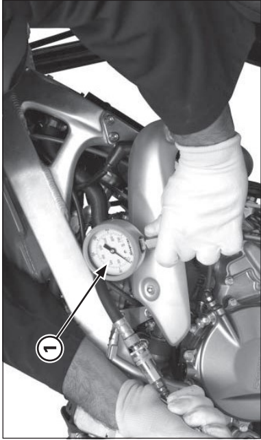
(1) CYLINDER COMPRESSION GAUGE
