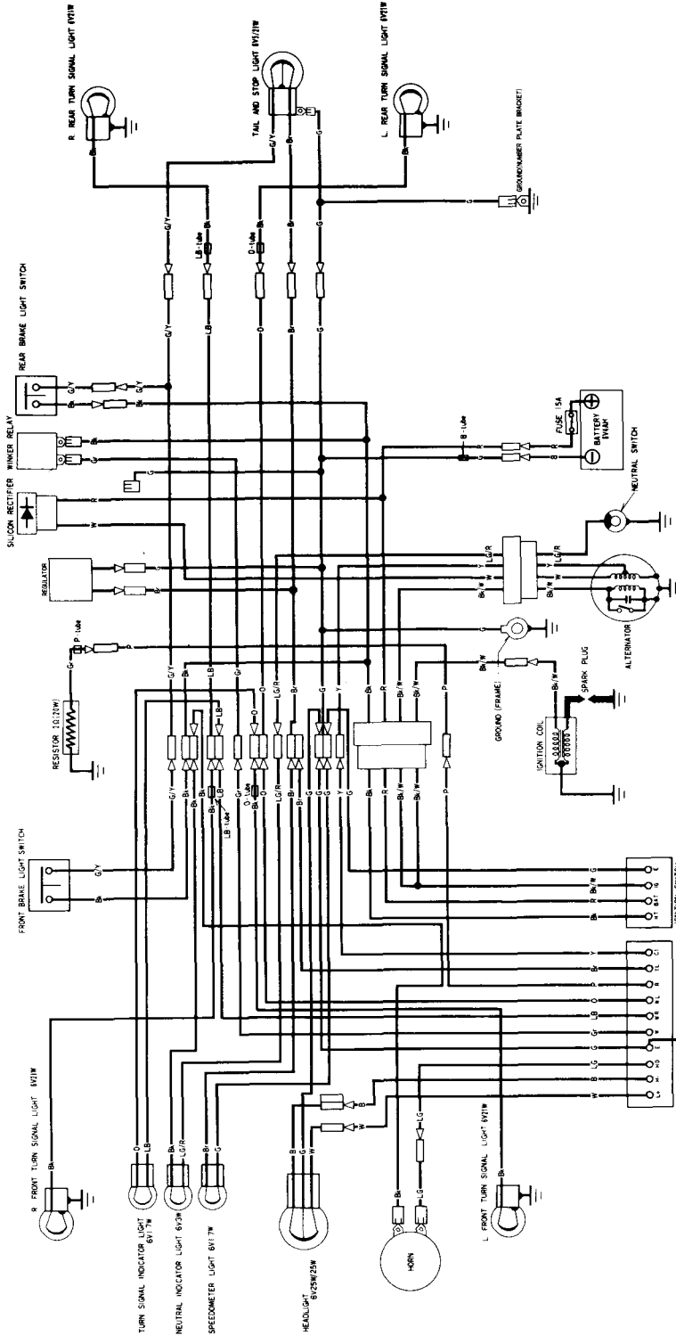
LIGHTING + DIMMER + TURN SIGNAL + HORN SWITCH
