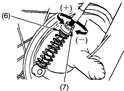
(6) lower lock nut (+) increase freeplay (7) lower adjusting nut (-) decrease freeplay
