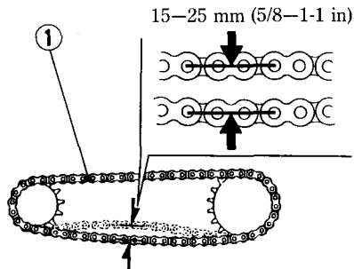
(1) Drive chain
