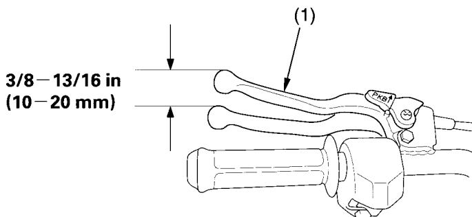
(1) rear brake lever
