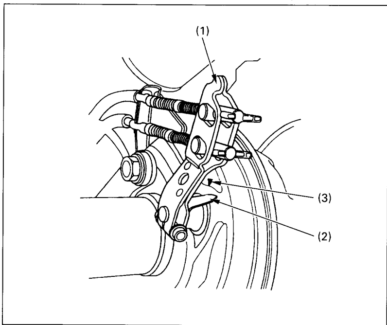
Fig. 4-23 (1) Brake arm
