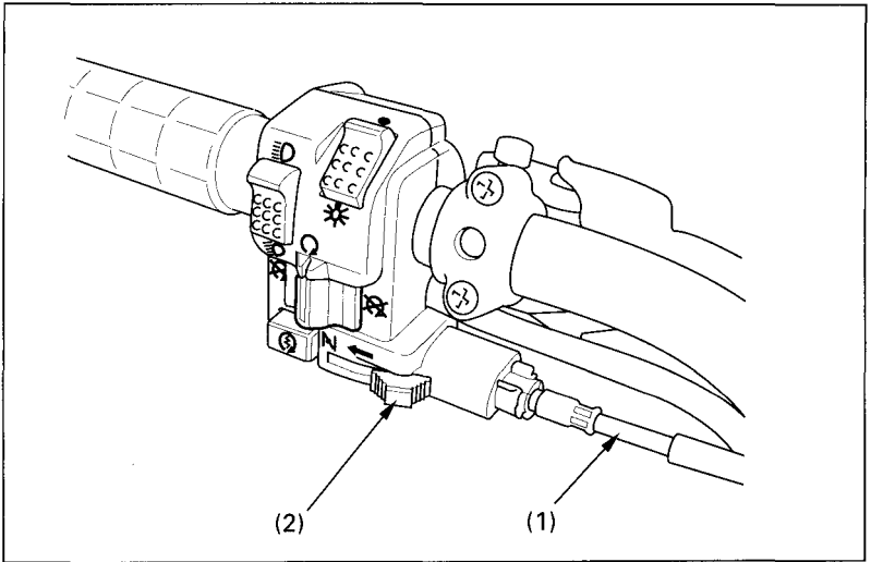
Fig. 4-8 (1) Choke cable
