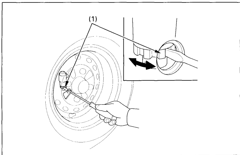
(1) Brake adjusters
