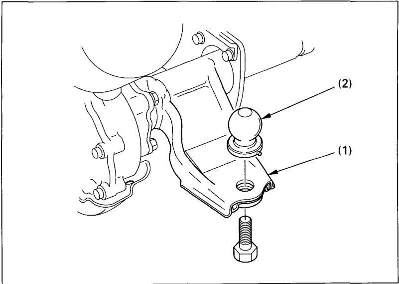
Fig. 2-30 (1) Trailer hitch
