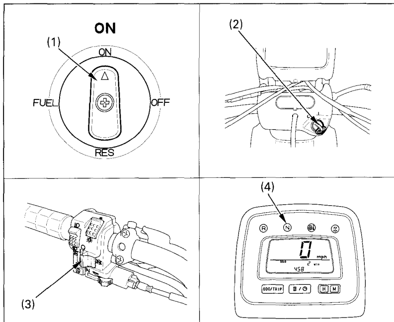
(3) Engine stop switch (4) Neutral indicator
