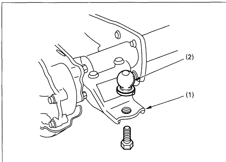
Fig. 2-30 (1) Trailer hitch
