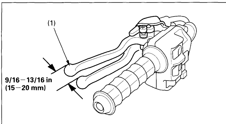
(1) Brake lever
