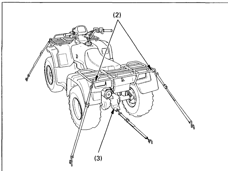
Fig. 4-42 Points to secure FOURTRAX with tie downs
