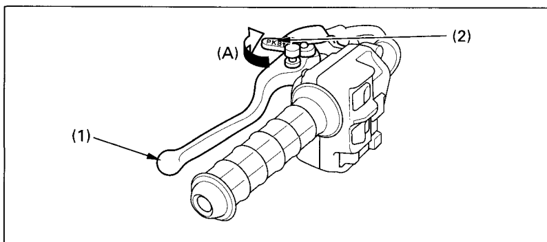
Fig. 2-24 (1) Rear brake lever/ Parking brake lever (2) Lock lever (A) To lock
