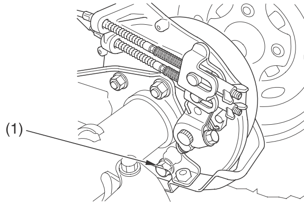
(1) rear brake drain bolt
