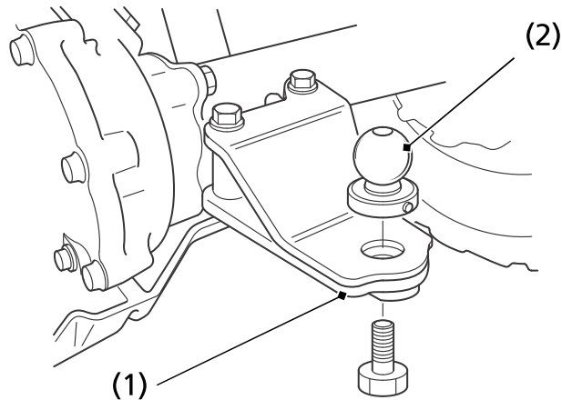
(1) trailer hitch
