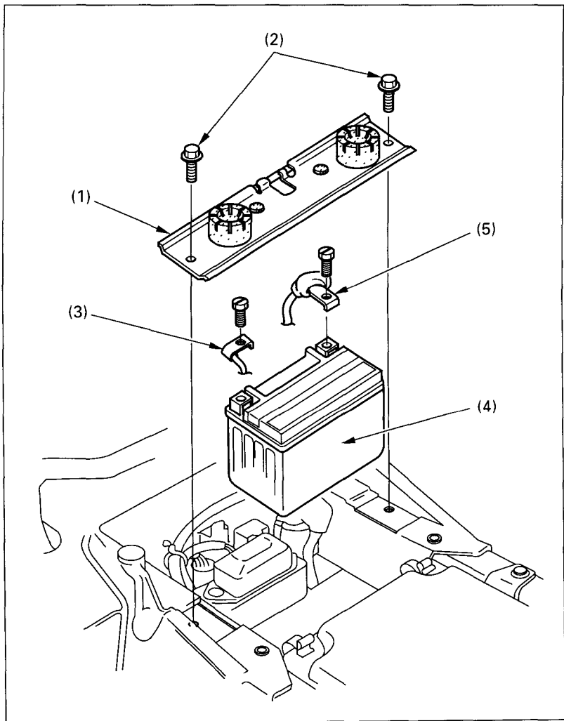
Fig. 4-19 (1) Battery holder (2) Mount bolts (3) Negative (-) terminal lead
