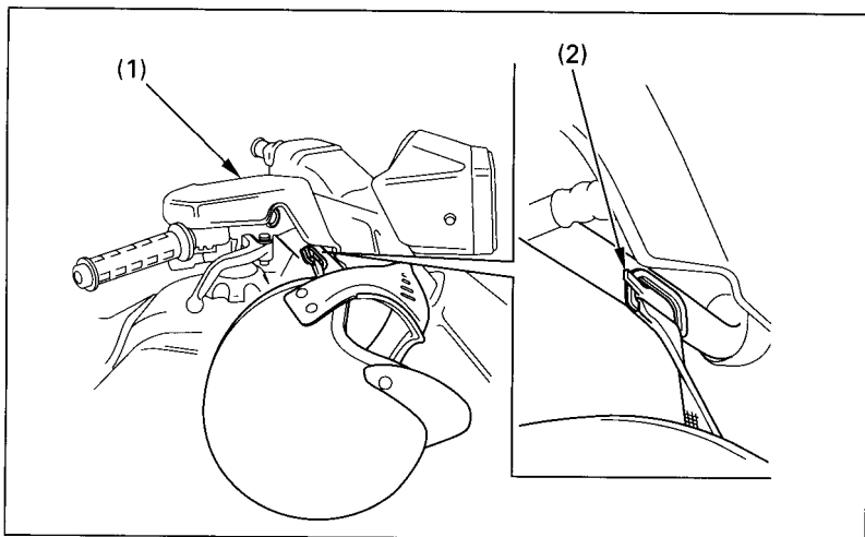
Fig. 2-23 (1) Handlebar cover
