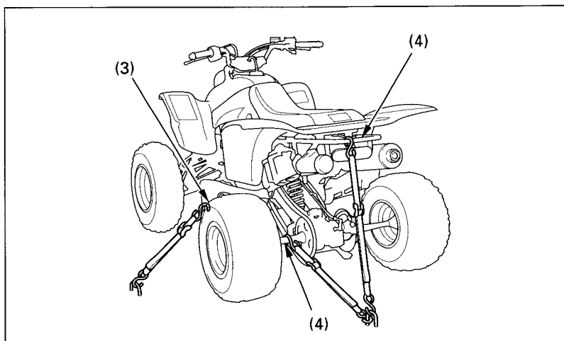
Fig. 4-37 Points to secure FOURTRAX with tie downs
