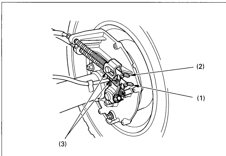
Fig. 4-27 (1) Brake pedal adjusting nut (2) Brake lever adjusting nut (3) Brake arm pin
