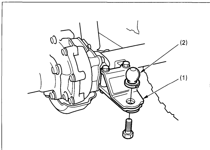
Fig. 2-29 (1) Trailer hitch
