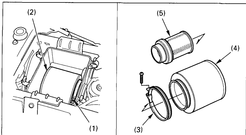
Fig. 4-5 (1) Screw (2) Air cleaner assembly (3) Clamp (4) Air cleaner (5) Air cleaner body
