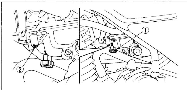
Fig. 4-9 (1) Throttle stop screw (2) Pilot screw
