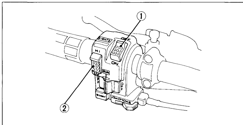
Fig. 2-12 (1) Headlight switch (2) Dimmer switch
