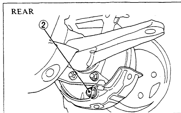
(2) Drain bolt
