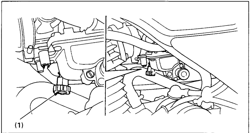
Fig. 4-10 (1) Throttle stop screw
