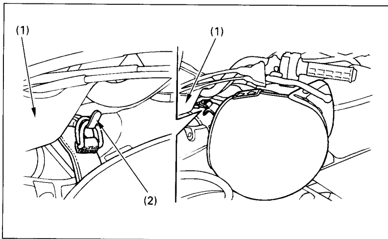
Fig. 2-25 (1) Handlebar cover (2) Helmet holder
