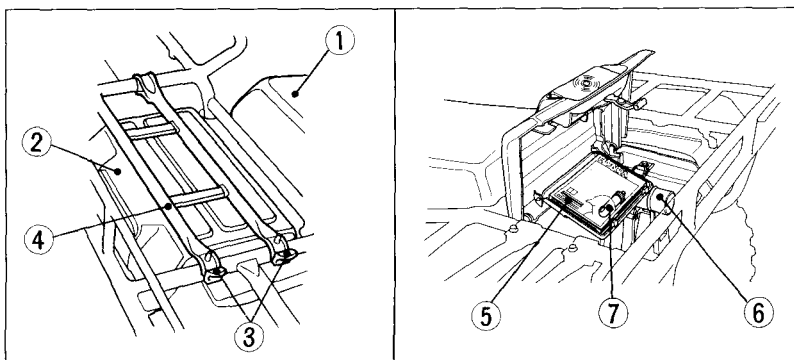
Fig. 2-23 (1) Seat (2) Storage compartment (3) Rubber straps (4) Rear rack (5) Owner's manual (6) Tool kit (7) Air pressure gauge
