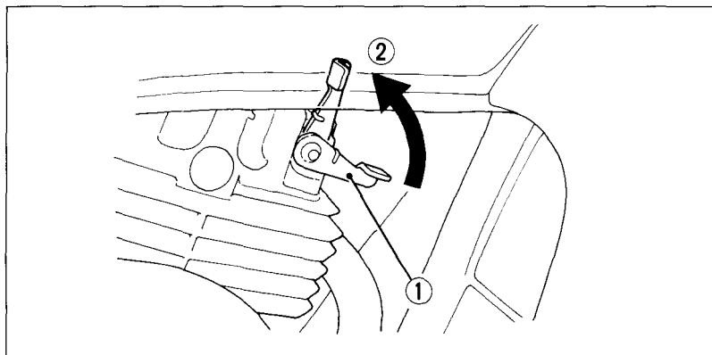
Fig. 2-10 (1) Decompression lever (2) "Decomp" position
