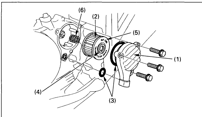
Fig. 4-12 (1) Oil filter cover (4) Rubber seal (2) Oil filter (5) OUT-SIDE mark (3) O-rings (6) Spring
