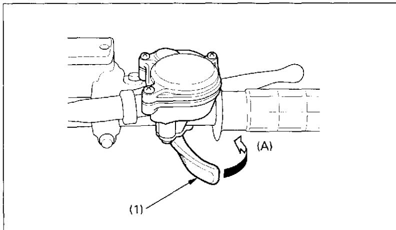
Fig. 2-12 (1) Throttle lever
