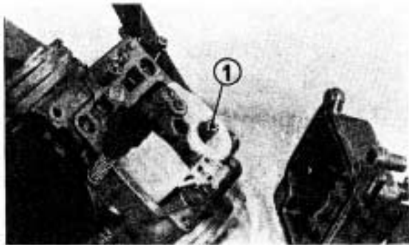
(1) Main jet
