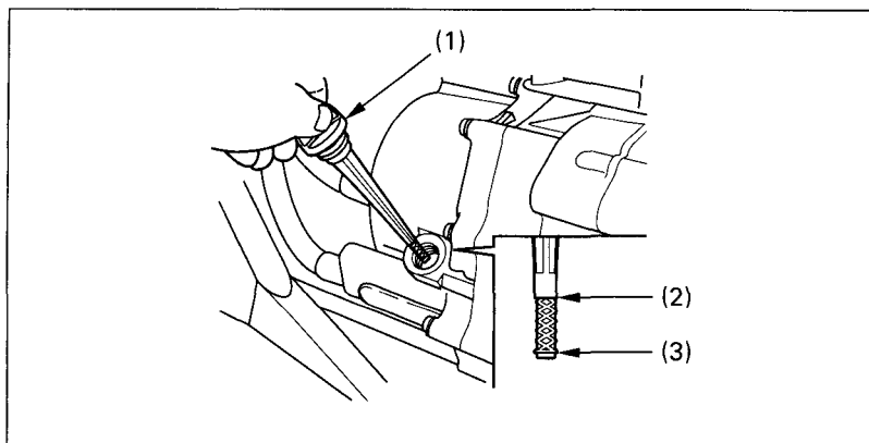
Fig. 2-16 (1) Oil filler cap/dipstick (2) Upper level mark (3) Lower level mark
