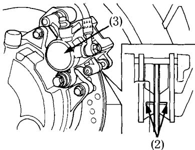
(3) Rear brake caliper (2) Wear line
