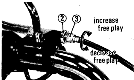
(2) Lock nut
