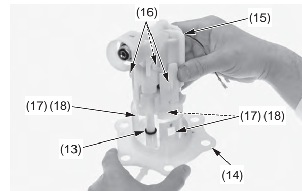
(13) new O-ring (14) fuel pump base (15) fuel pump unit holder assembly (16) hooks (17) grooves (18) tabs
