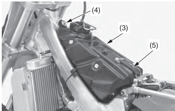
(3) fuel tank (5) fuel tank band (4) collar and fuel tank bolt
