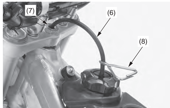
(6) breather tube (8) hose clamp (7) steering stem nut
